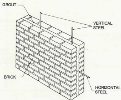
REINFORCED BRICK MASONRY
