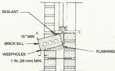
Sill in Cavity Wall Construction FIG. 10
