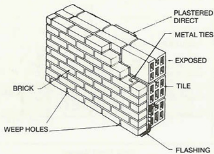
METAL-TIED SOLID WALLS
