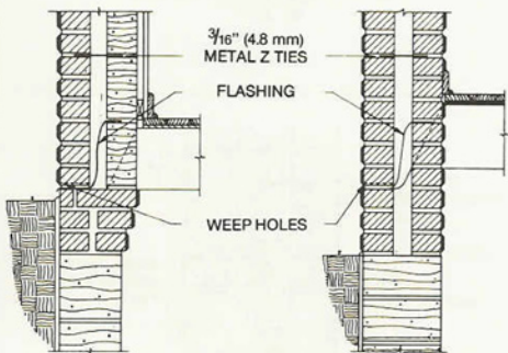
Foundation Details FIG. 8
