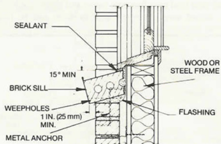
Sill in Frame/Brick Veneer Construction FIG. 9
